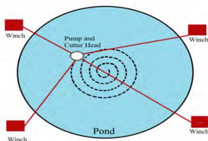
Standard Dredge Pattern
