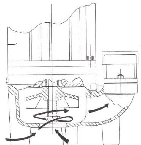
SL-1000 (P50CSD) with Dredging Auger
