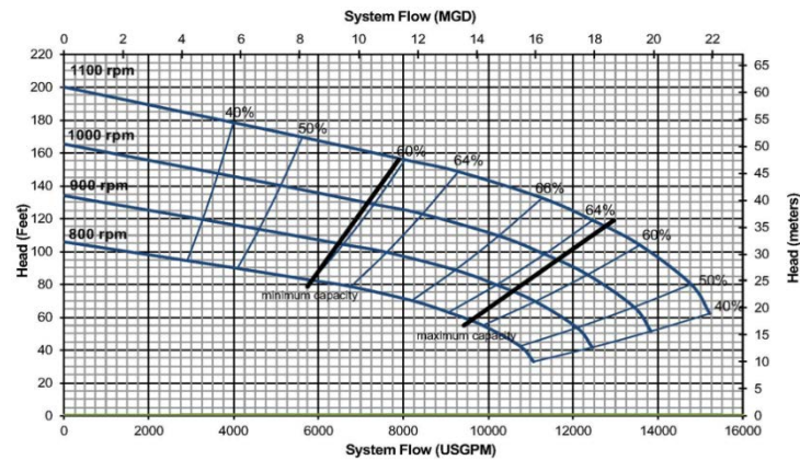
Godwin CD500M 64% efficient at BEP
