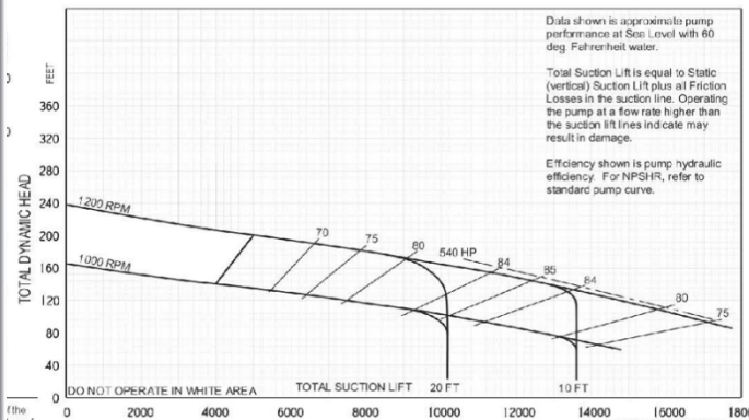
Mighty Pumps DT18 85% efficient at BEP
